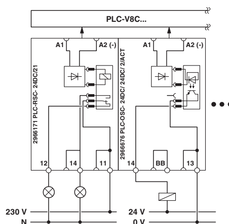
Circuit diagram
